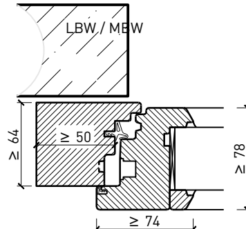
Blockrahmen 74 mm
