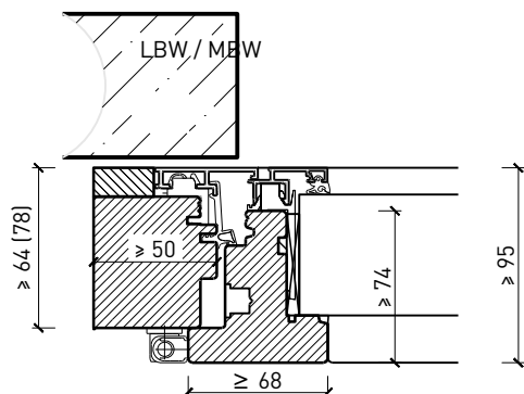
Blockrahmen 64 (78) mm
