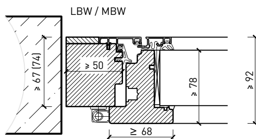
Blockrahmen 67 (74) mm
